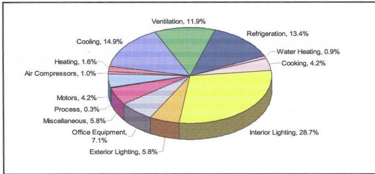
Figure E-3: Electric Usage by End Use
