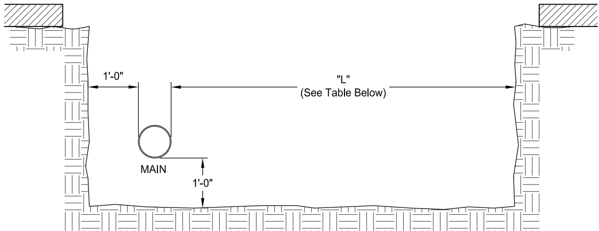
SECTION VIEW
