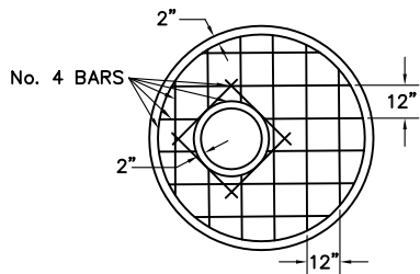
FLAT SLAB TOP
