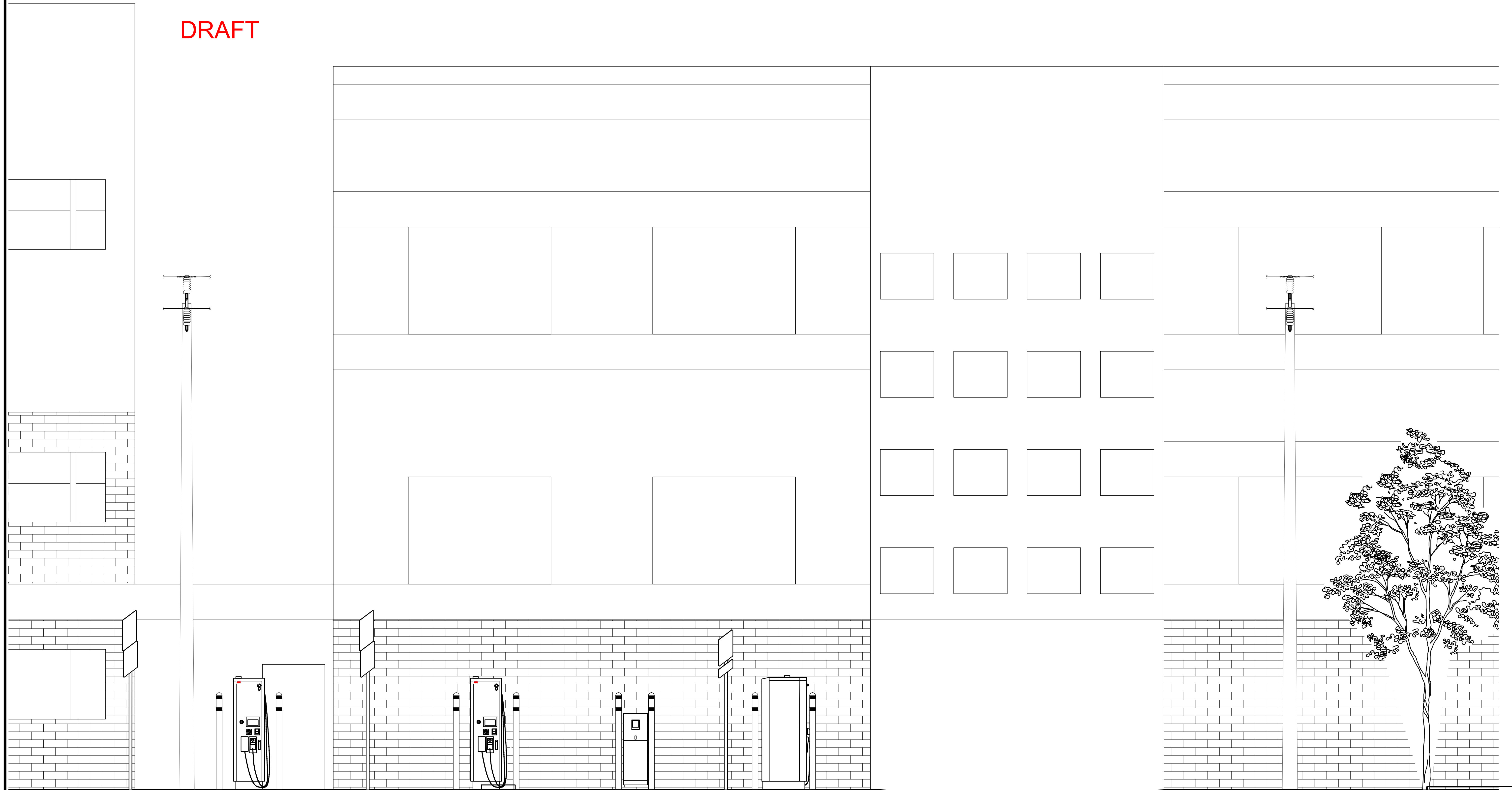
A EQUIPMENT SITE ELEVATION G.5 SCALE: 3/8" = 1'-0"
