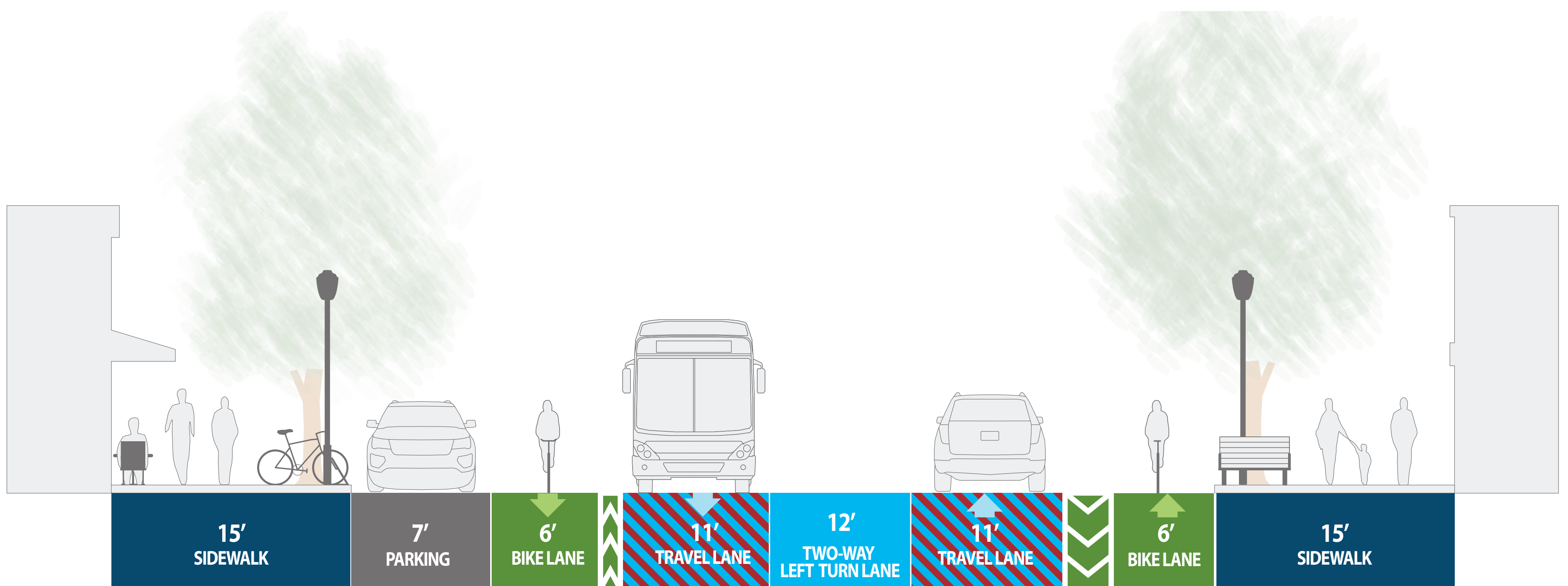
ROAD DIET WITH BUFFERED BIKE LANES WITH CENTER TURN LANE 36th Street to 38th Street
